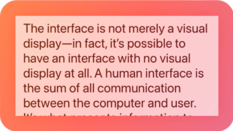
Text views
