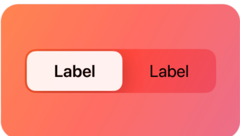
Segmented controls
