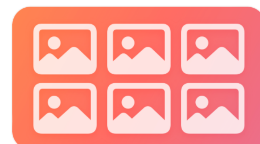
Collections
