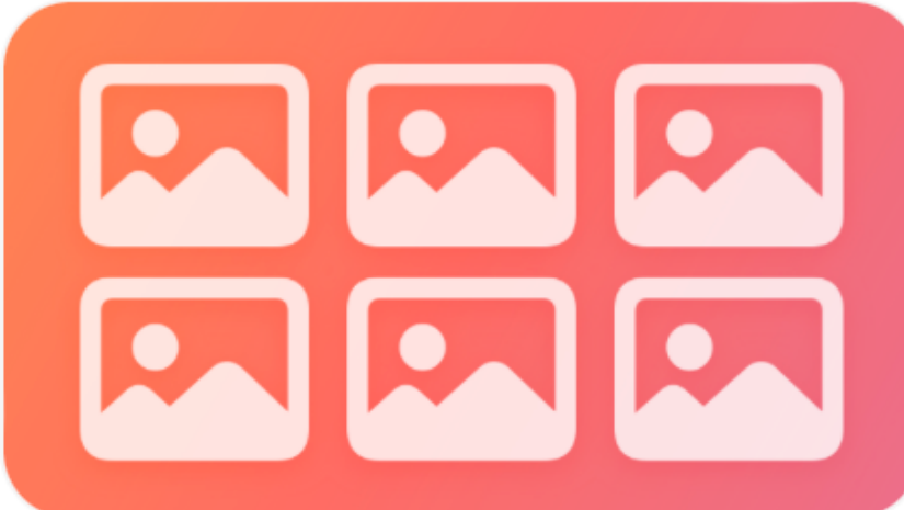
Collections
