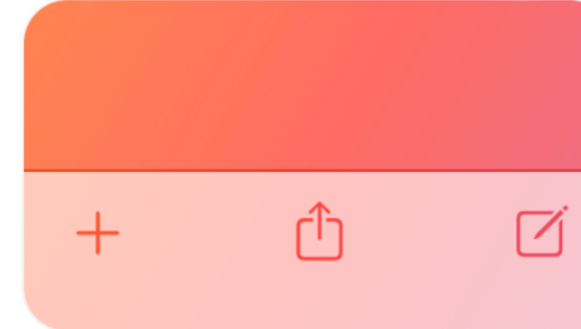
Toolbars
