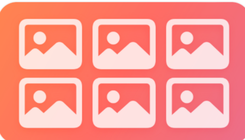
Collections
