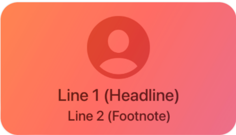
Lockups
