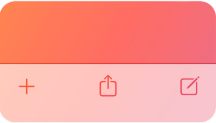
Toolbars
