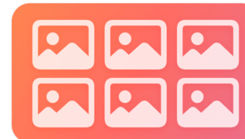
Collections
