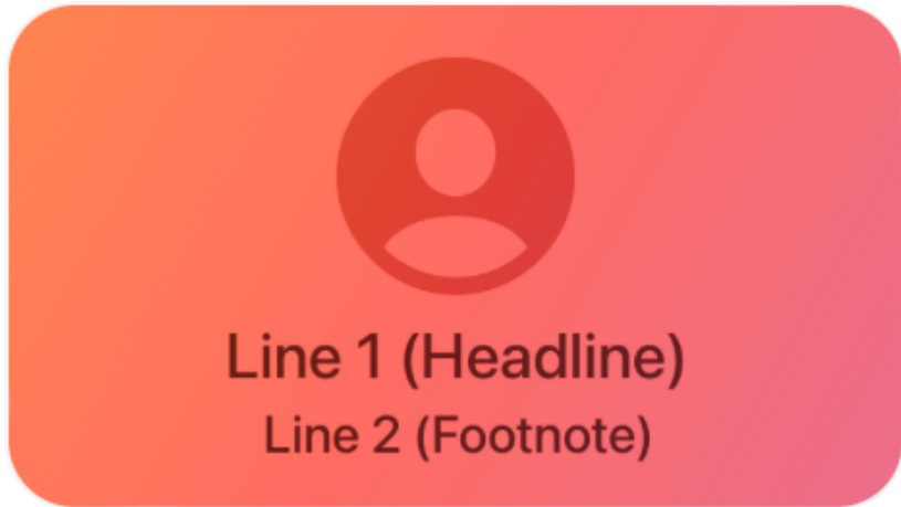
Lockups
