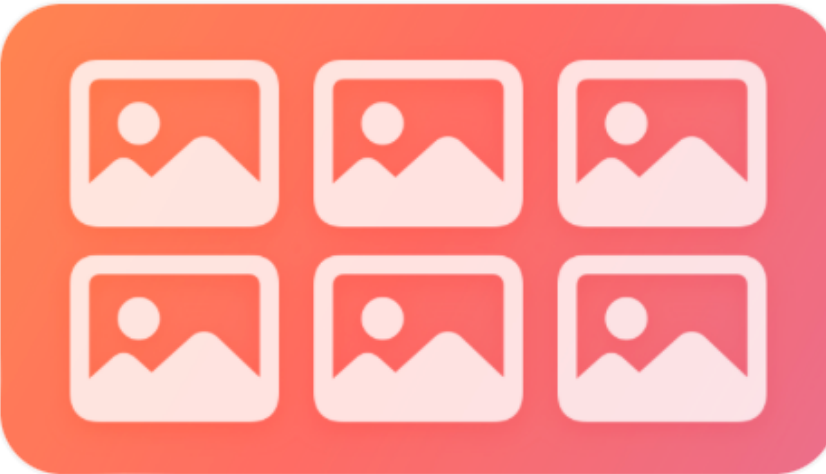
Collections
