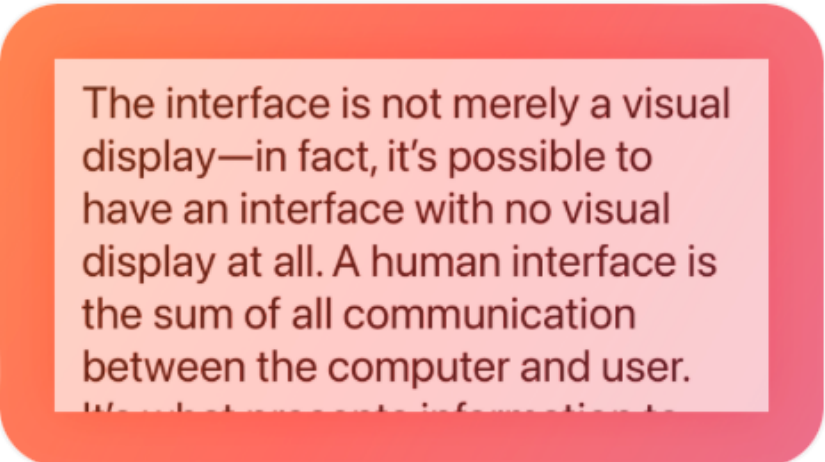
Text views
