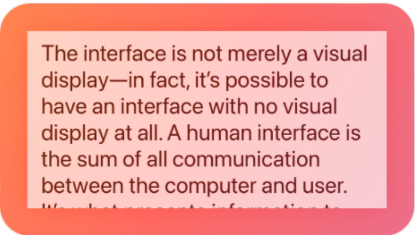
Text views
