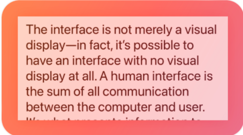
Text views
