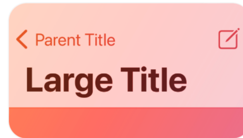
Navigation bars
