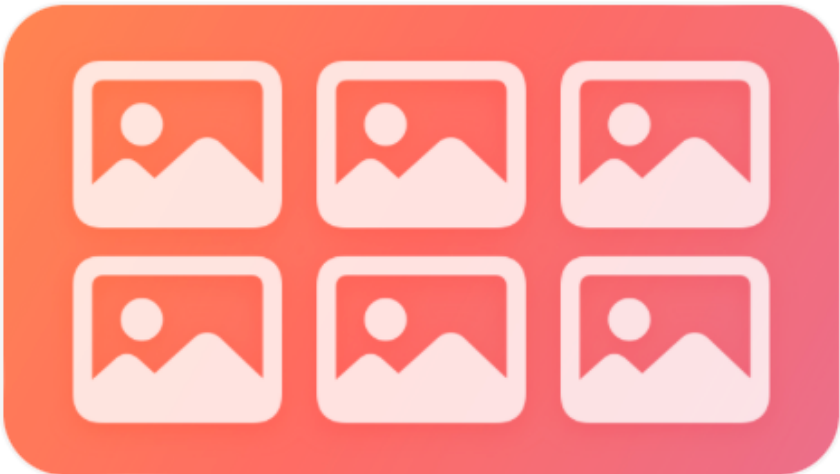
Collections
