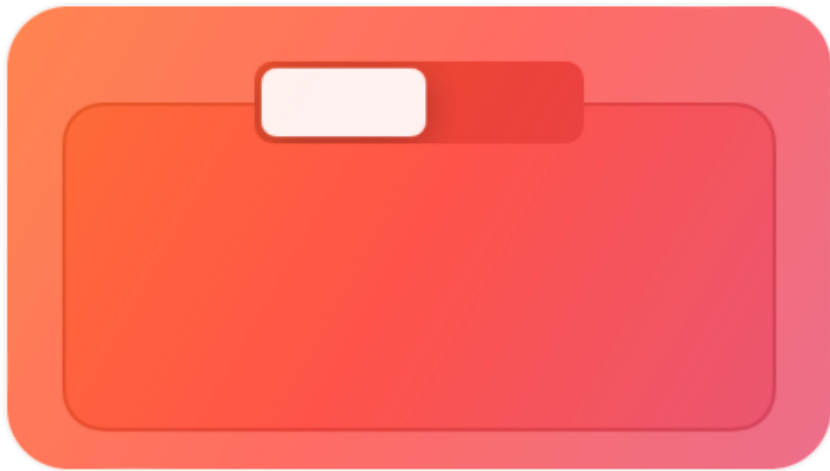
Tab views
