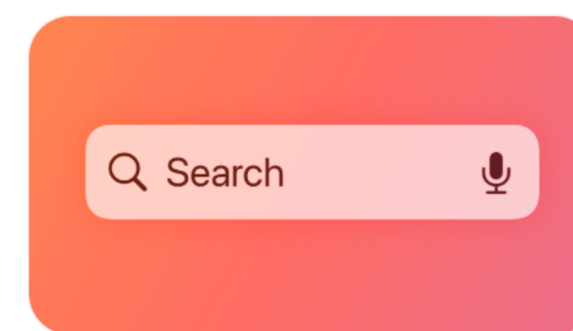
Search fields
