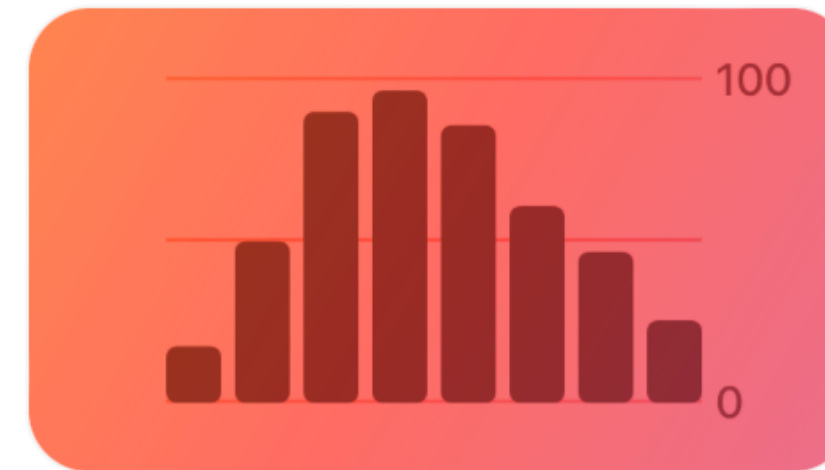
Charts
